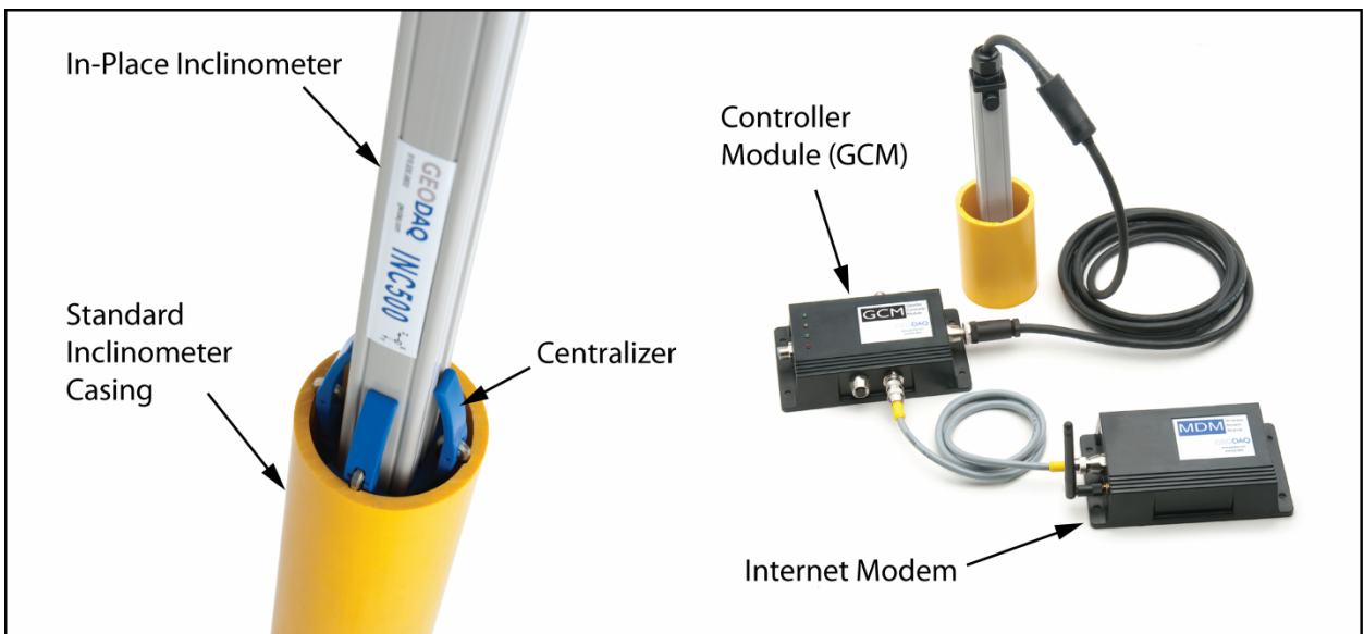
Figure 7. In-Place Incliner and Data Collection Hardware
