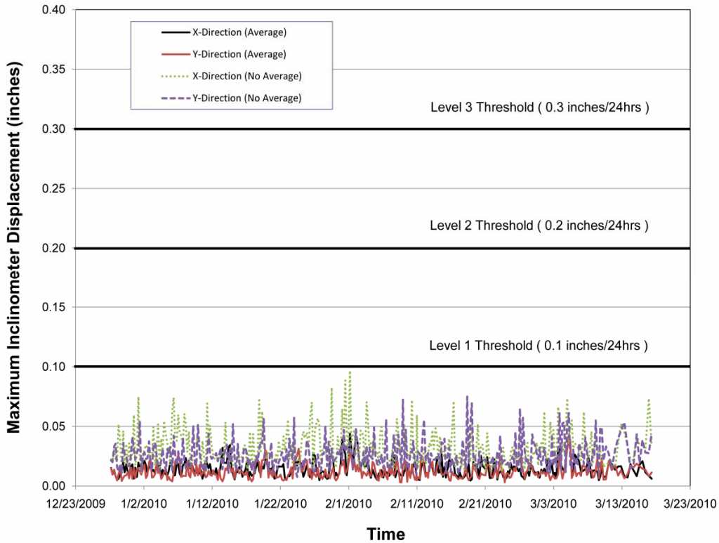
Figure 11. Maximum Displacements for 24-Hour Period, Inclinometer I-4
