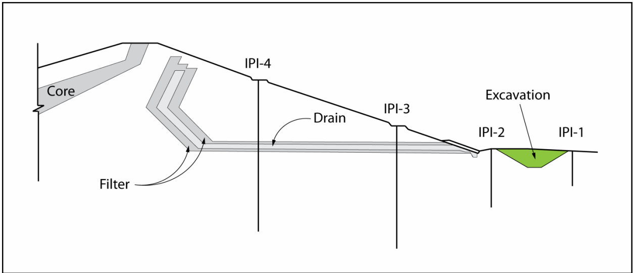
Figure 6. In-Place Incliner Elevations for IPI-1, IPI-2, IPI-3 and IPI-4
