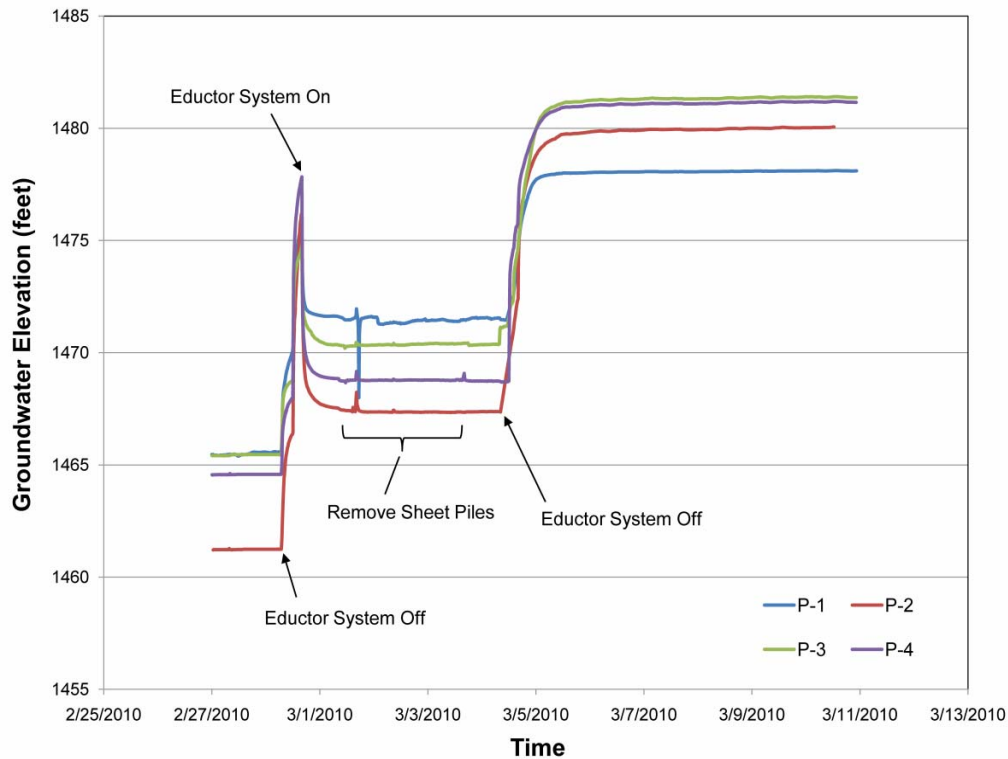
Figure 9. Typical Piezometer Readings
